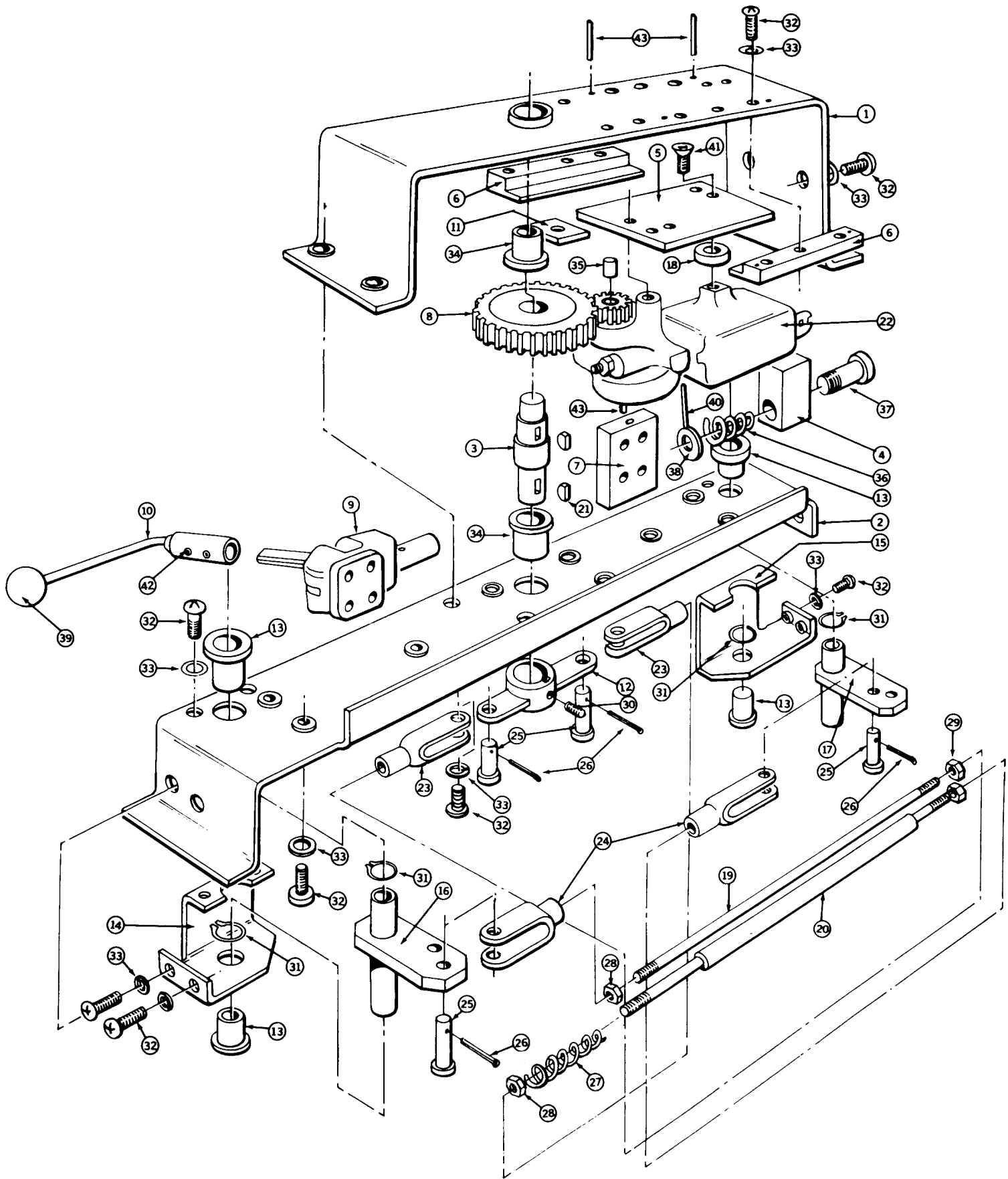
FIGURE 1 — Excell Shuttle-Bus Door Mechanism Model 7189-001
